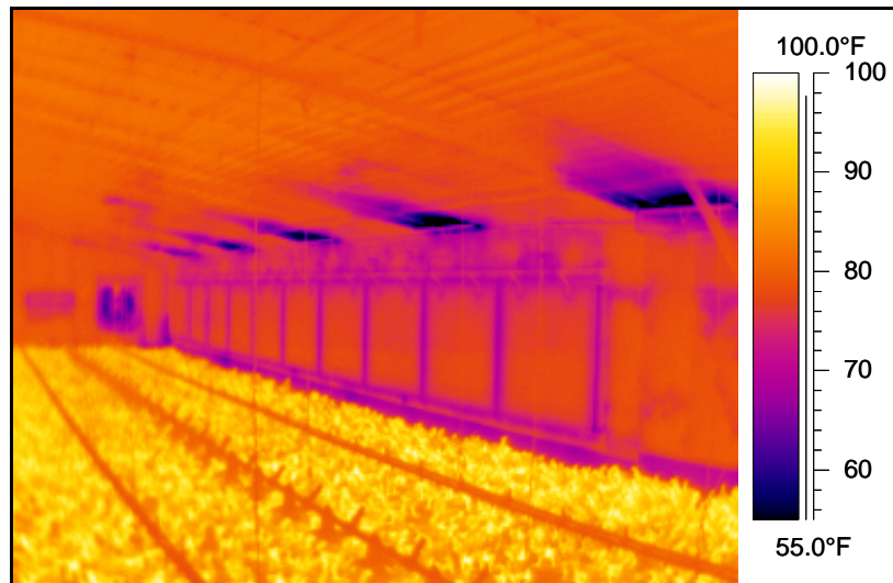
Figure 3. Fresh air entering only through air inlets (very tight house)
