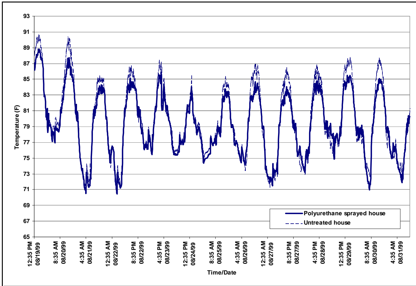
Figure 3. Air temperatures at fan end of the houses
