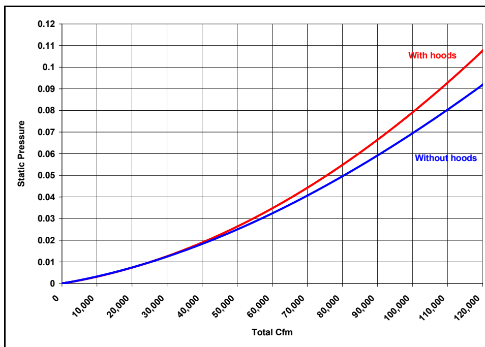
Figure 12. Total fan cfm vs Static pressure
