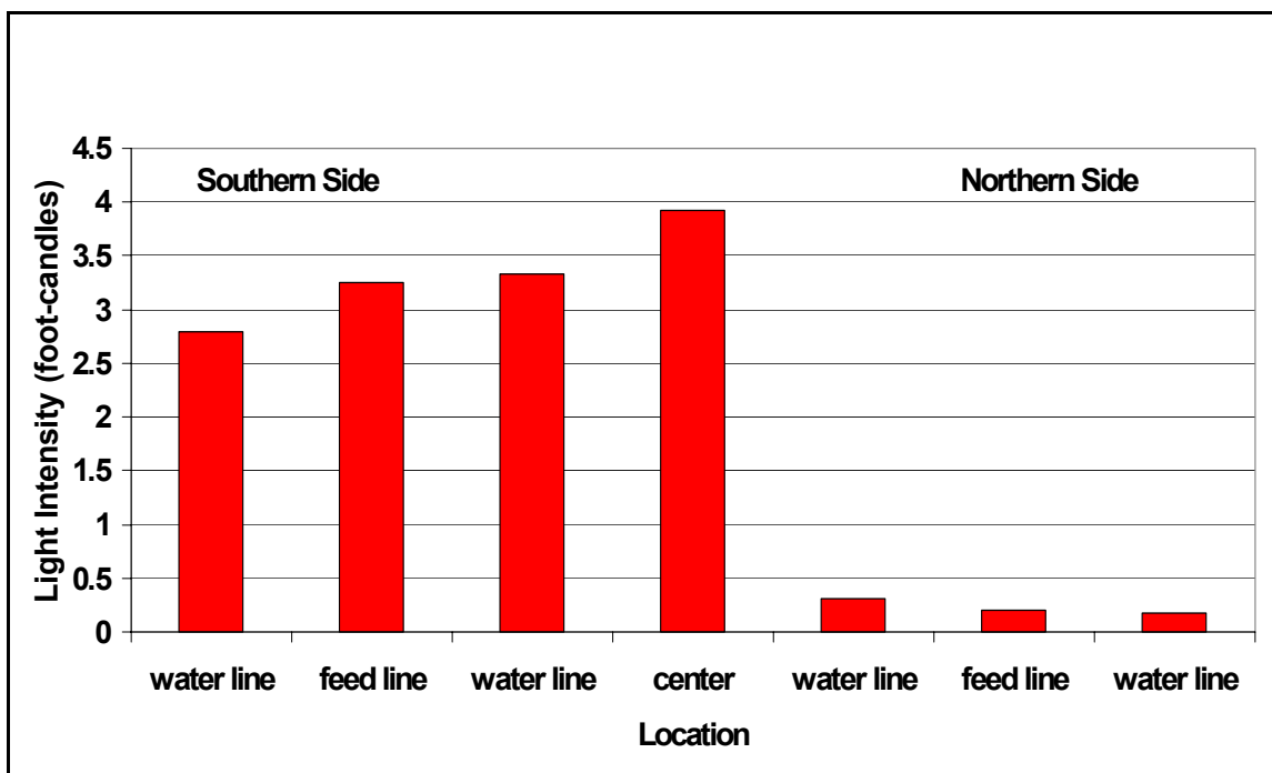
Figure 11. Early morning light intensity in house without hoods.
