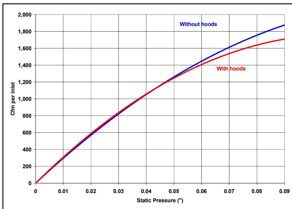
Figure 13. Cfm per inlet Vs. Static pressure
