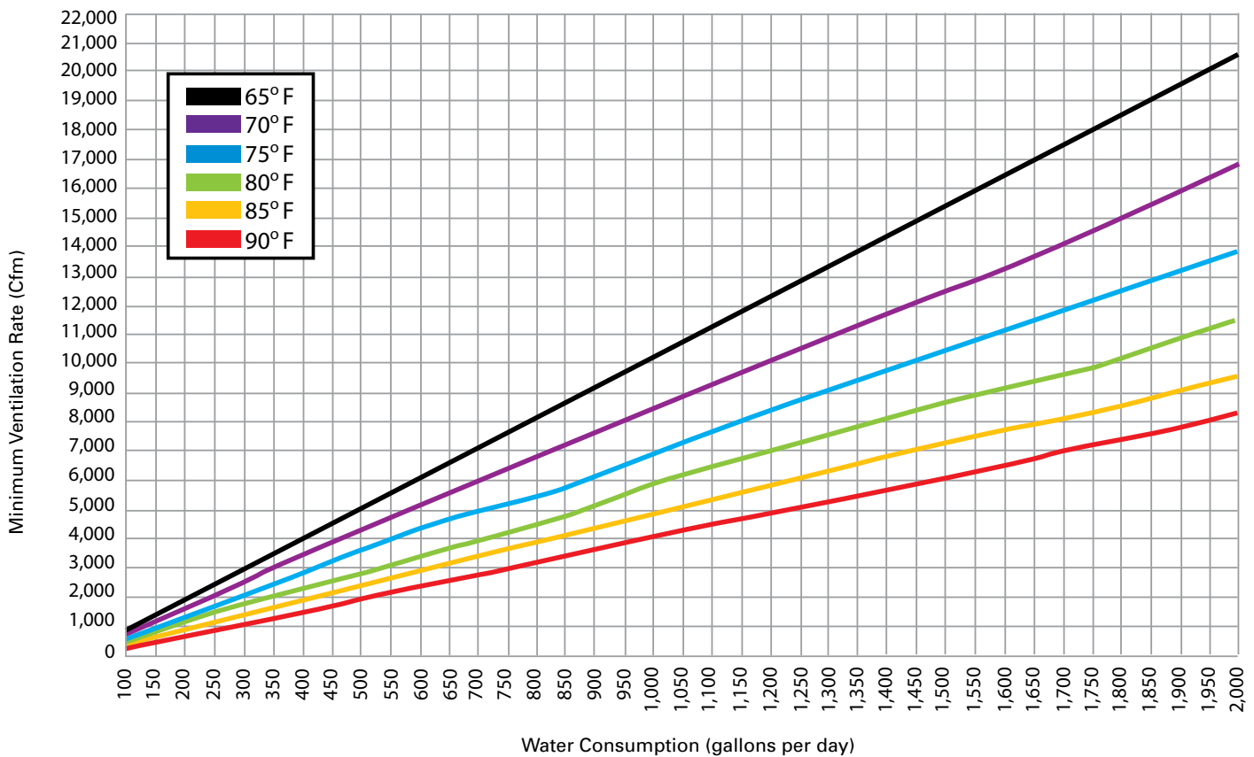
Figure 2. Minimum ventilation rates required to manage house moisture based on bird water usage and inside temperature
